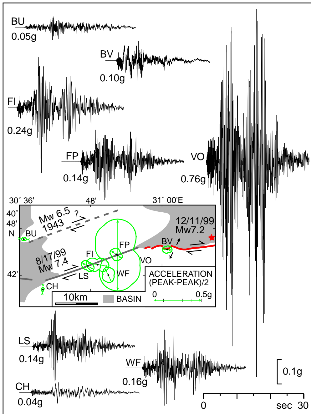
Horizontal motion from the 12 Nov 1999 Mw7.2 Duzce earthquake (surface rupture in red) in northwestern Turkey recorded by the Karadere network (inset map). Rose diagrams ( in green) centered at each station represent the azimuthal distribution of maximum horizontal (P-P)/2 acceleration. FBA seismograms show horizontal acceleration in the direction of maximum peak-to-peak values (marked by double arrow in rose diagrams). SEEBER ET AL., 2000.
